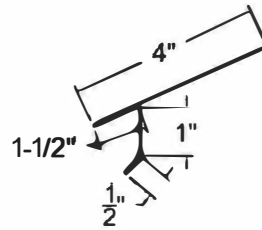
DRIP EDGE (PITCH REQUIRED)
