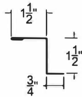
RAKE CLEAT "Z" CLOSURE
