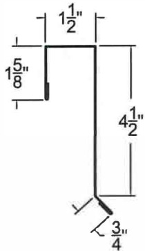
HIDDEN FASTENER RAKE
