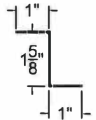
RIDGE & END WALL "Z" CLOSURE
