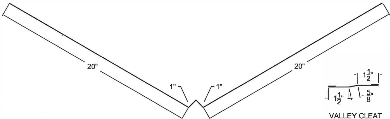
VALLEY "W" FLASHING
