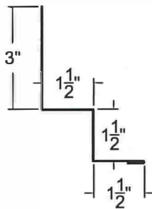
EXPOSED FASTENER SIDEWALL FLASHING
