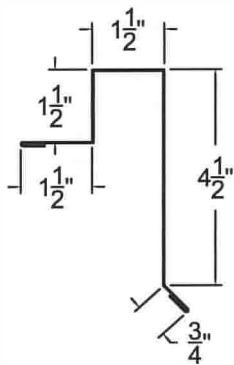
EXPOSED FASTENER RAKE
