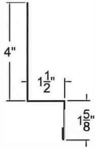
HIDDEN FASTENER SIDEWALL FLASHING
